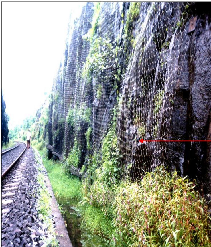
STEEL BOULDER NET
