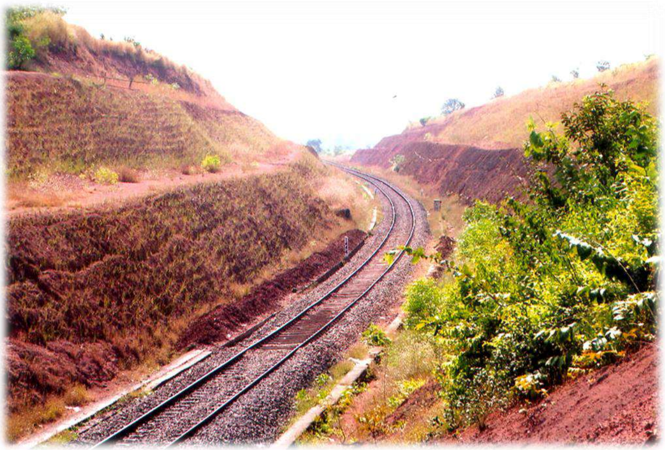
Vetiver Plantation on Soil Cutting Slopes for prevention of Soil erosion
